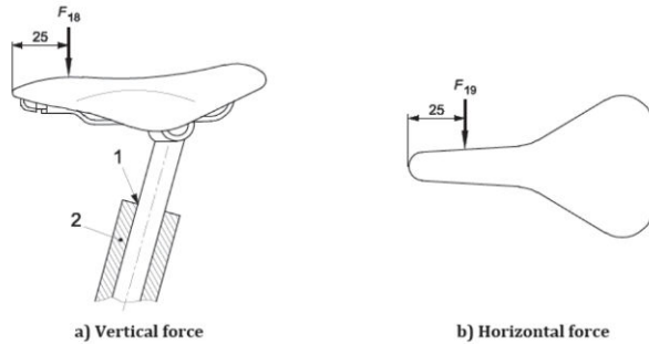
Figure 48 — Saddle/seat-post: safety test
