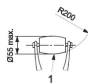
Figure 26 — Low-mass roller
