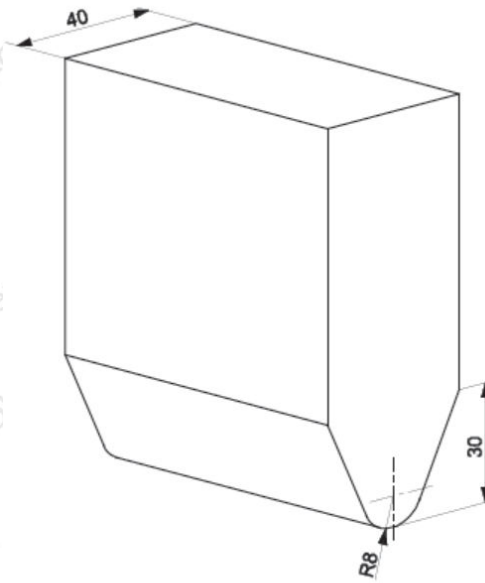
Figure 39 — Striker dimensions
